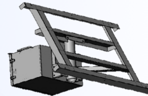
Metal Pole Solar Panel Mount and Insulated Battery Box
